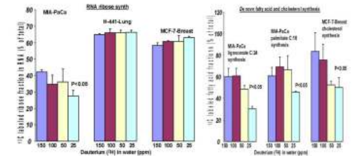
FIGURE 5. Limited RNA 13 C labeling is closely associated with the limited synthesis of nuclear membrane lignocerate (C24:0) in MIA-PaCa and cholesterol in breast cancer cells.
